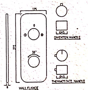
FLR-5681K Aquamax Exposed Part Kit of Thermostatic Shower Mixer with 2-way diverter (Suitable for ALD-681)
