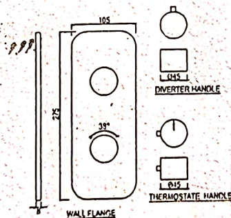
FLR-5661K Aquamax Exposed Part Kit of Thermostatic Shower Mixer (Suitable for ALD-661)
